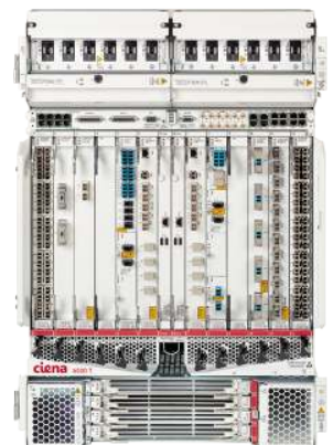
Figure 2. 6500-T12 shelf equipped with 500G/slot switching modules
